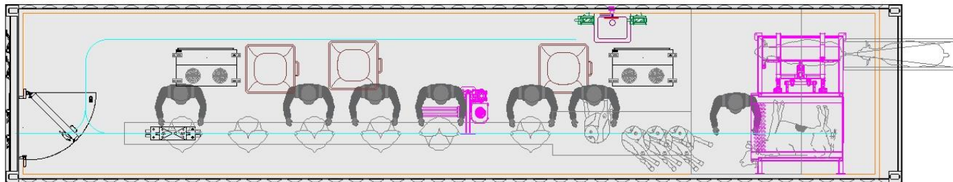
SHEEP SLAUGHTERING UNIT - T2 +18°C 10-15 Sheep/hour
